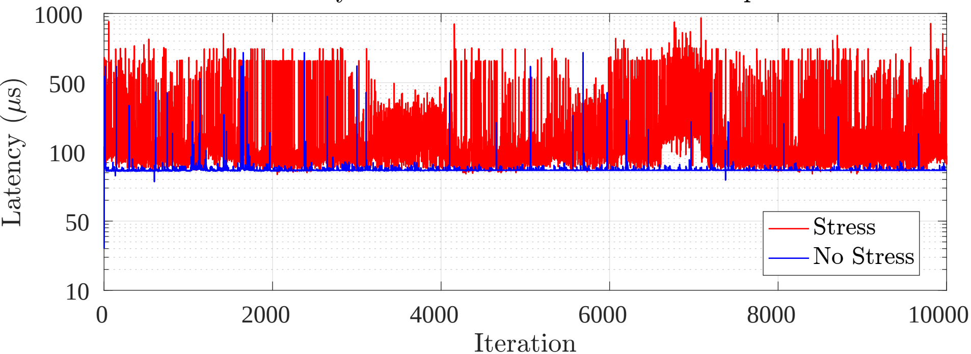
Latency for Scheduler: SCHED_OTHER p99
